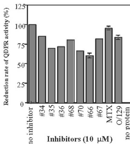
FIG. 7. Tests of pteridine analogs for inhibition of purified recombinant LmQDPR . qDPR activity was assayed in the presence of the indicated inhibitors whose structures can be found in Ref. 39. The results are expressed as percentage reduction activity with respect to a control without inhibition. The mean \pm S.D. from three experiments are shown.
