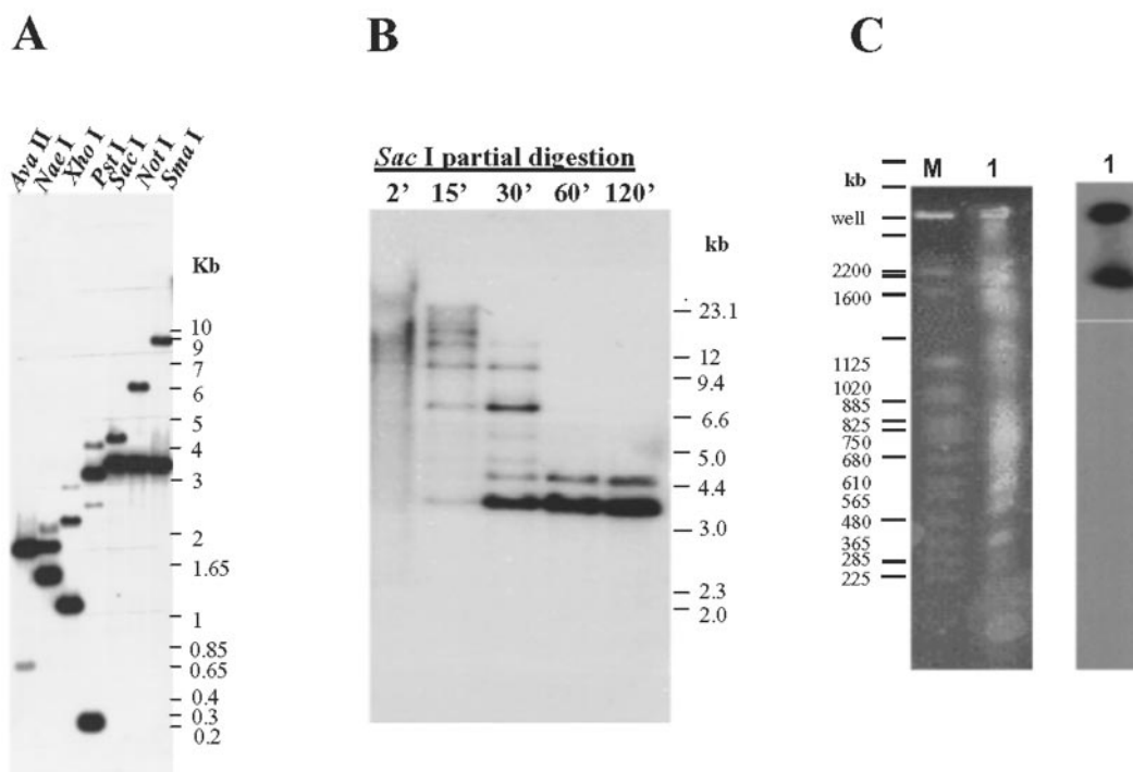
FIG. 3. Southern blot analysis of the genomic organization of L. major QDPR. In all panels, the hybridization probe was the LmQDPR ORF probe shown in Fig. 4A. A. Southern blot. L. major genomic DNA was completely digested with the indicated restriction enzymes, electrophoresed on a 0.8% agarose gel, blotted, and hybridized. The sizes of the molecular weight markers are shown. B. partial digestion with Sac I. A standard digestion of L. major genomic DNA was initiated (0.5 unit of Sac I, 7 \mu g of genomic DNA), and at the intervals indicated aliquots were withdrawn and the reactions stopped by adding EDTA (to 15 mM) and quick-freezing. Samples were electrophoresed on a 0.8% agarose gel, blotted, and hybridized. C. chromosomal mapping of QDPR. L. major chromosomes were resolved by pulsed field gel electrophoresis as described under "Experimental Procedures," blotted, and hybridized. The left panel shows the ethidium bromide-stained gel with S. cerevisiae chromosomal markers in kb (M), and the right panel shows the autoradiogram.
