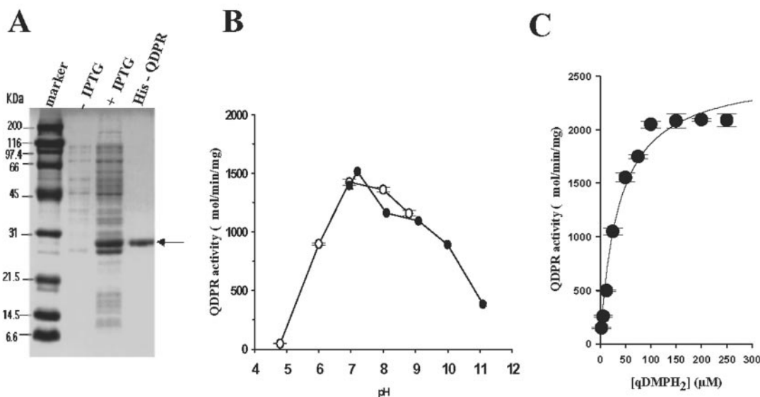
FIG. 6. Expression and characterization of recombinant L. major QDPR. A, purification of LmQDPR from E. coli . Samples were electrophoresed through a 15% SDS-polyacrylamide gel, and the gel was stained with Coomassie Brilliant Blue. Lane 1, molecular mass markers (in kDa); lane 2, crude extract of uninduced E. coli ; lane 3, E. coli lysate after isopropyl-1-thio- \beta -D-galactoside induction; and lane 4, protein recovered after Ni 2+ -nitrilotriacetic acid-agarose chromatography. The arrow indicates His 6 -QDPR. B, pH profile. qDPR activity assays were performed with recombinant L. major QDPR (30 ng of purified recombinant protein/ml, 100 \mu M NADH, 100 \mu M DMPH 4 ) using two overlapping buffers at the indicated pH. \circ , 50 mM sodium phosphate, and \bullet , 50 mM Tris-HCl. The values shown are the average of three independent experiments \pm S.D. C, substrate dependence of qDPR activity. The activity of purified recombinant LmQDPR was assayed at the indicated concentrations of qDMPH 2 .
