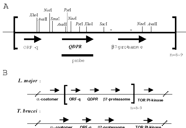
FIG. 4. The L. major QDPR repeating unit contains two other genes while the syntenic region of T. brucei lacks QDPR. A, map of the consensus L. major QDPR repeating unit. This was assembled from individual shotgun sequences as described in the text and is shown linearized arbitrarily at a Bsa BI site (GenBank™ accession numbers AF523363 and AY141854). Arrows show the coding regions for ORF-q, QDPR, and the 20 S proteasome \beta 7 subunit. A, “*” indicates polymorphic sites as discussed in the text. B, comparison of the organization of the QDPR locus of L. major with a syntenic region of T. brucei . Preliminary contigs spanning the LmQDPR region or its equivalent in T. brucei were prepared using information deposited in GenBank™ or generously made available by the Leishmania and T. brucei genome projects (see “Acknowledgments”). The predicted gene order is shown; these regions are syntenic except for the absence of the QDPR in T. brucei . The contigs and specific sequence information used in their assembly are available from the authors by request.
