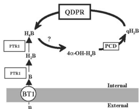
FIG. 1. Proposed enzymatic pathways for the consumption and regeneration of H_4B in Leishmania . B, biopterin; qH_2B , quinonoid-dihydrobiopterin; 4\alpha\text{-OH-H}_4B , pterin- 4\alpha -carbinolamine; and "?", predicted activity, either an unidentified enzyme or spontaneous oxidation.
