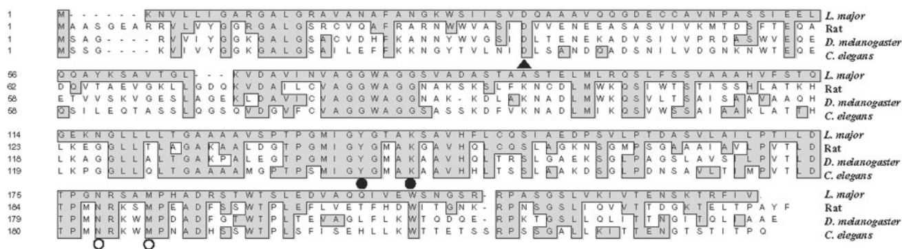
FIG. 2. Alignment of eukaryotic qDPRs . An amino acid sequence alignment of qDPRs from L. major (this work), rat (GenBank™ accession number P11348), C. elegans (T24395), and D. melanogaster (AAF50315) was performed using the Clustal algorithm implemented in the Lasergene software (DNASTAR, Inc.). Identical amino acids in all sequences are highlighted with a gray background. The residues interacting with NADH for hydride transfers are indicated by filled circles, the residues involved in substrate binding are indicated by open circles, and the residues involved in NADH binding preference are indicated by filled triangles (61–63).
