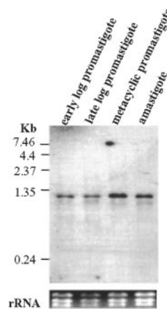
FIG. 5. Expression of QDPR mRNA during the Leishmania infectious cycle. Total RNAs (5 \mu g) were separated on a 1.5% formaldehyde-agarose gel, transferred to GeneScreen Plus, and hybridized with the QDPR probe (Fig. 4A). The autoradiogram is shown in the upper panel with the single \sim 1.1-kb QDPR transcript. Molecular weight standards (kb) are shown. The lower panel shows the ethidium bromide-stained gel region containing the three rRNAs as a loading control. Samples were RNAs from early logarithmic promastigotes (lane 1), late logarithmic promastigotes (lane 2), metacyclic promastigotes (lane 3), and amastigotes (lane 4).
